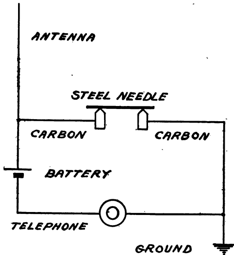
FIG. 12.—MICROPHONE CONNECTIONS.
